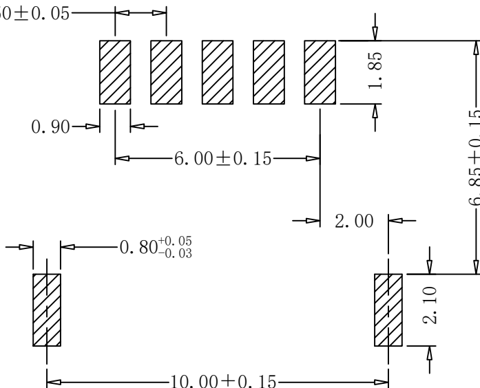
PCB LAYOUT
