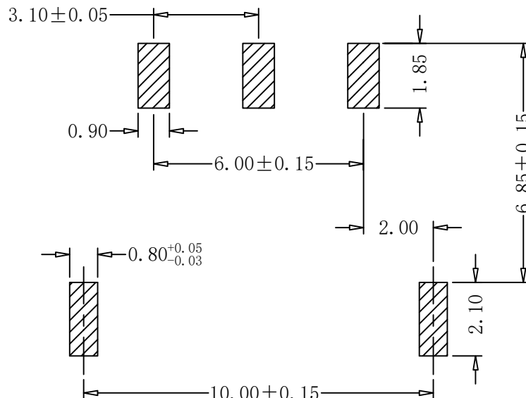
PCB LAYOUT
