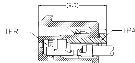
TER&amp;TPA Assembly Drawing
