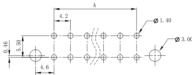
P. C. B LAYOUT
