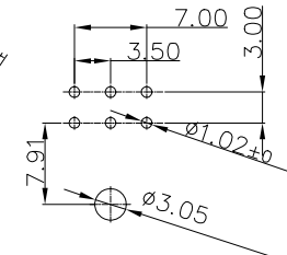
PCB Layout (2*2~2*3P)
